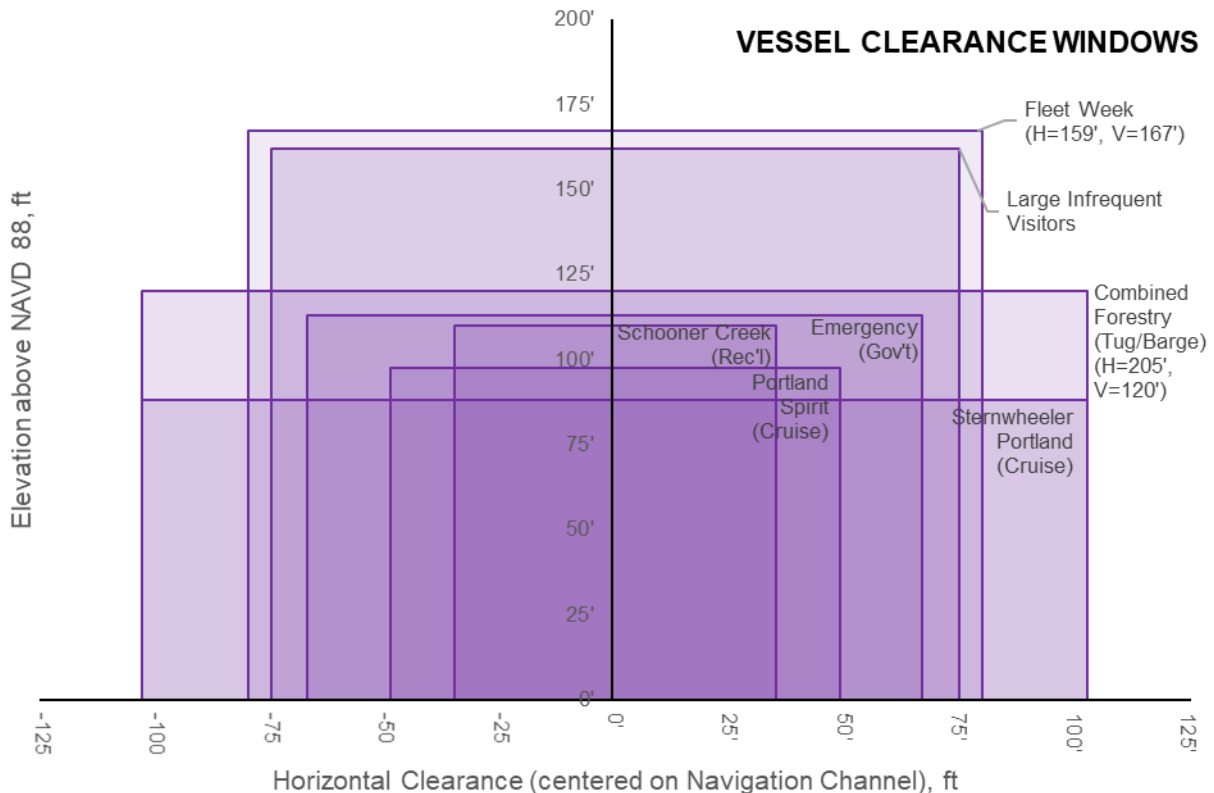
Figure 24. Elevation Requirement and Corresponding Horizontal Clearance Requirement for Each River User Type
